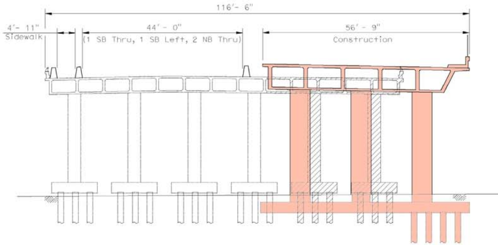
TYPICAL SECTION (STAGE 1 CONSTRUCTION)
