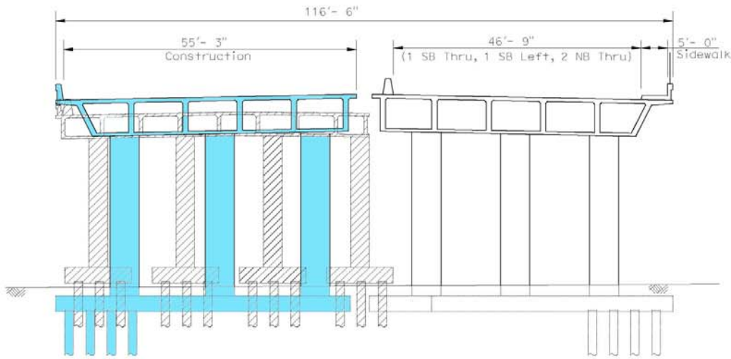
TYPICAL SECTION (STAGE 2 CONSTRUCTION)
