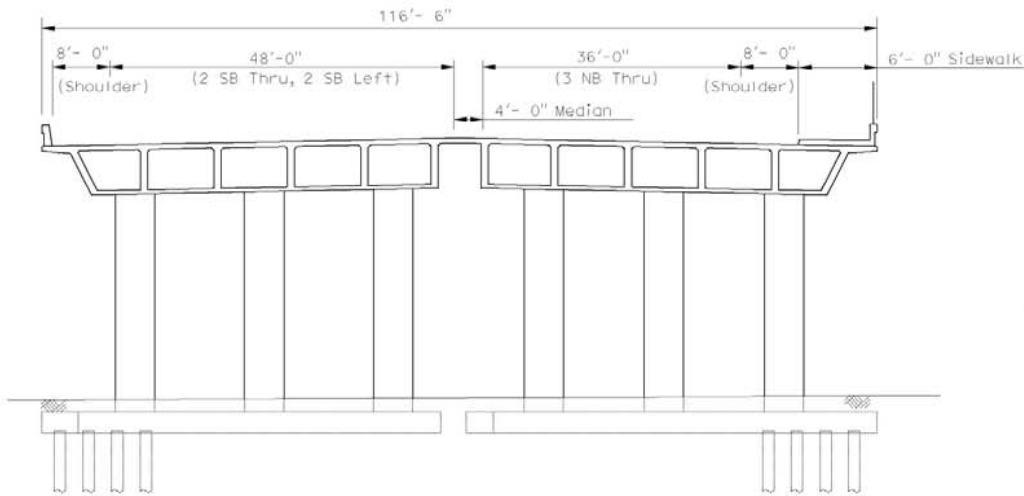
TYPICAL SECTION (FINAL CONFIGURATION)
