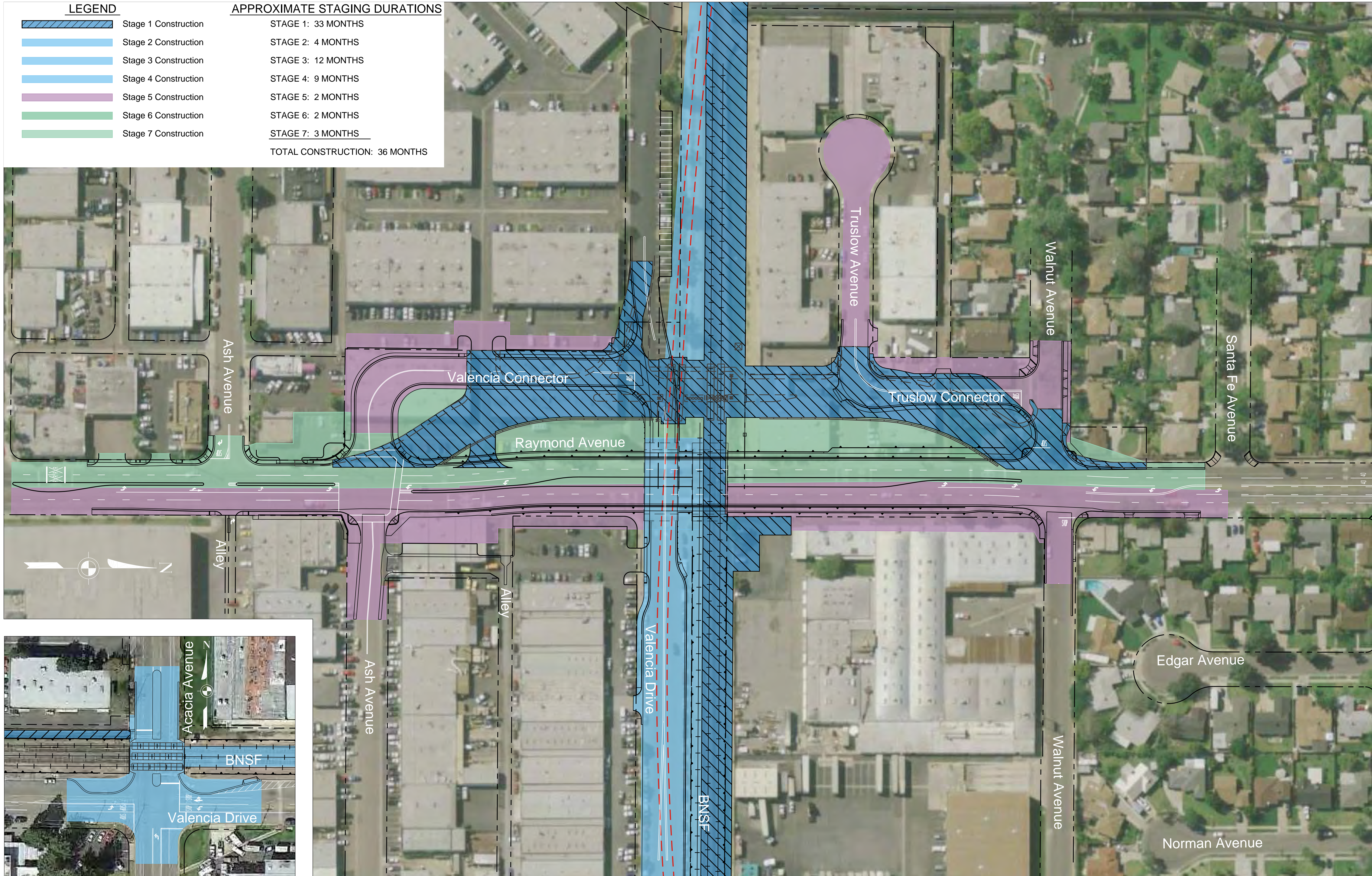
Raymond Avenue Grade Separation COMPOSITE CONSTRUCTION STAGING EXHIBIT
