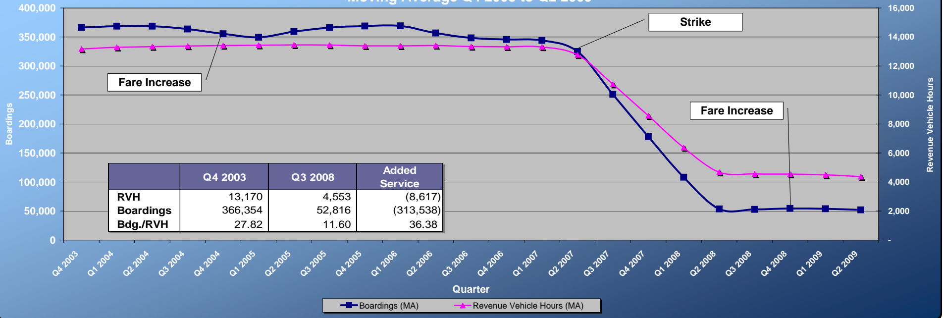
Boardings Vs. Revenue Vehicle Hours (EDO - Express Directly Operated) Moving Average Q4 2003 to Q2 2009
